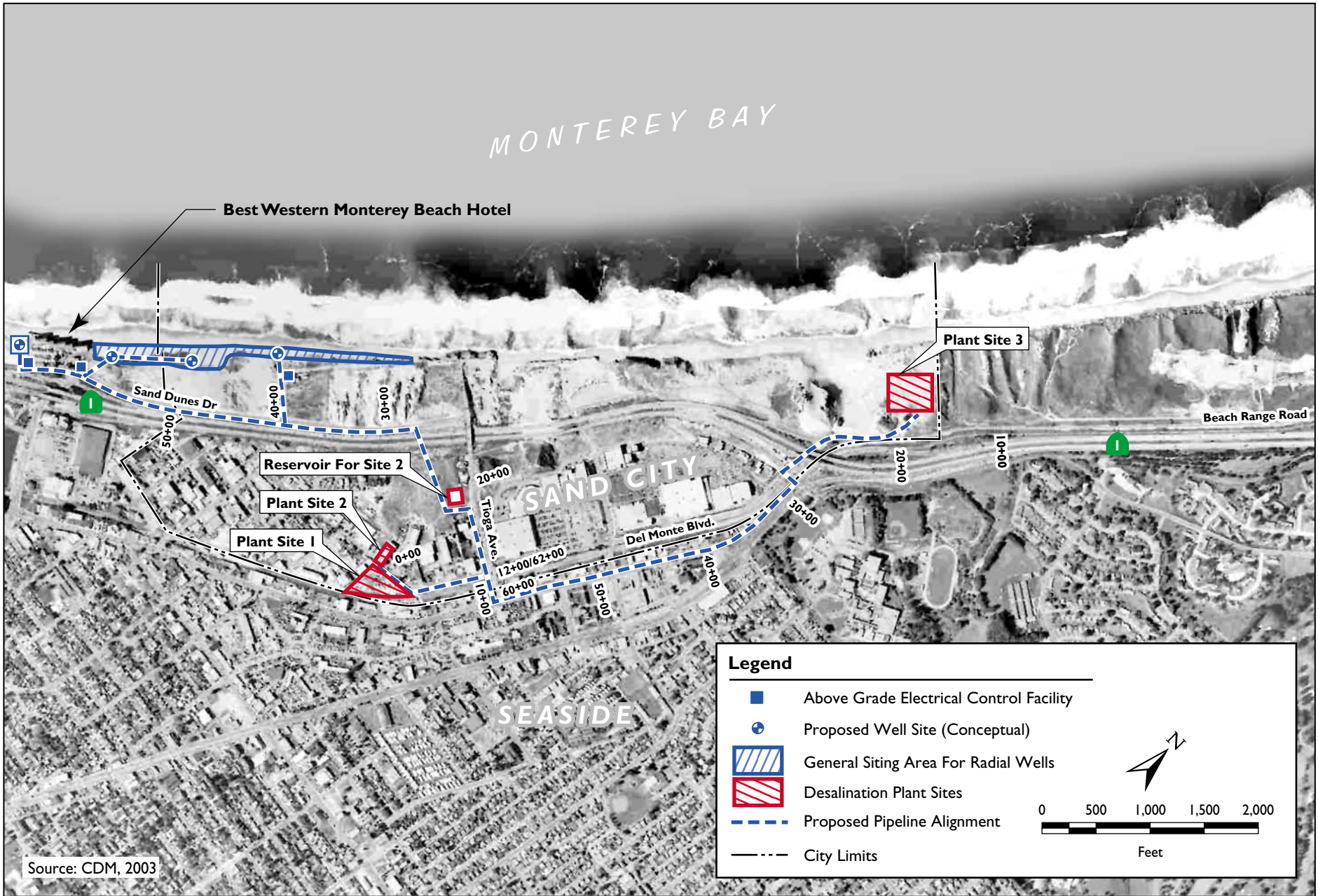
Figure ES-2 Location of Radial Wells and Collection Pipelines
