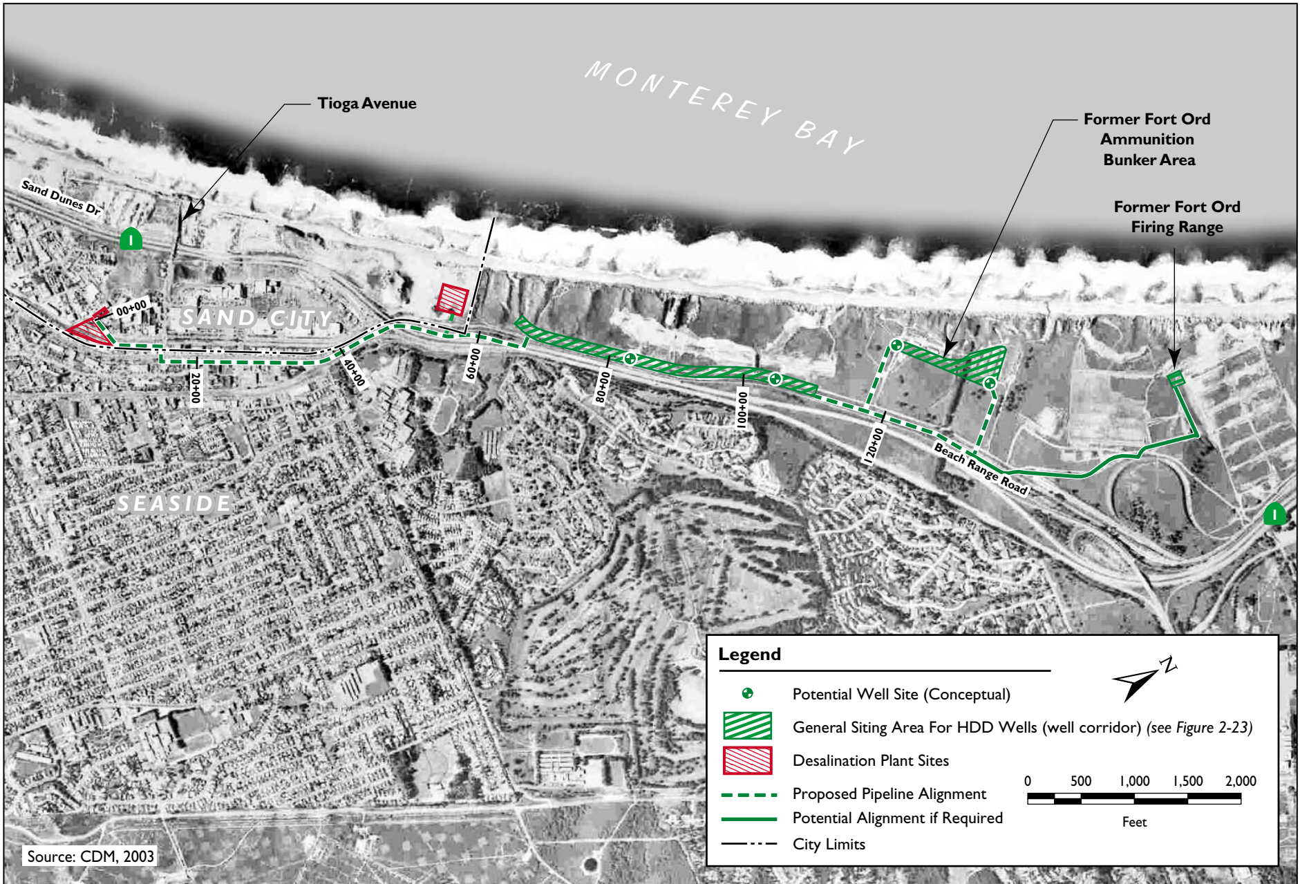
Figure ES-3 Location of Brine Disposal Wells and Pipelines
