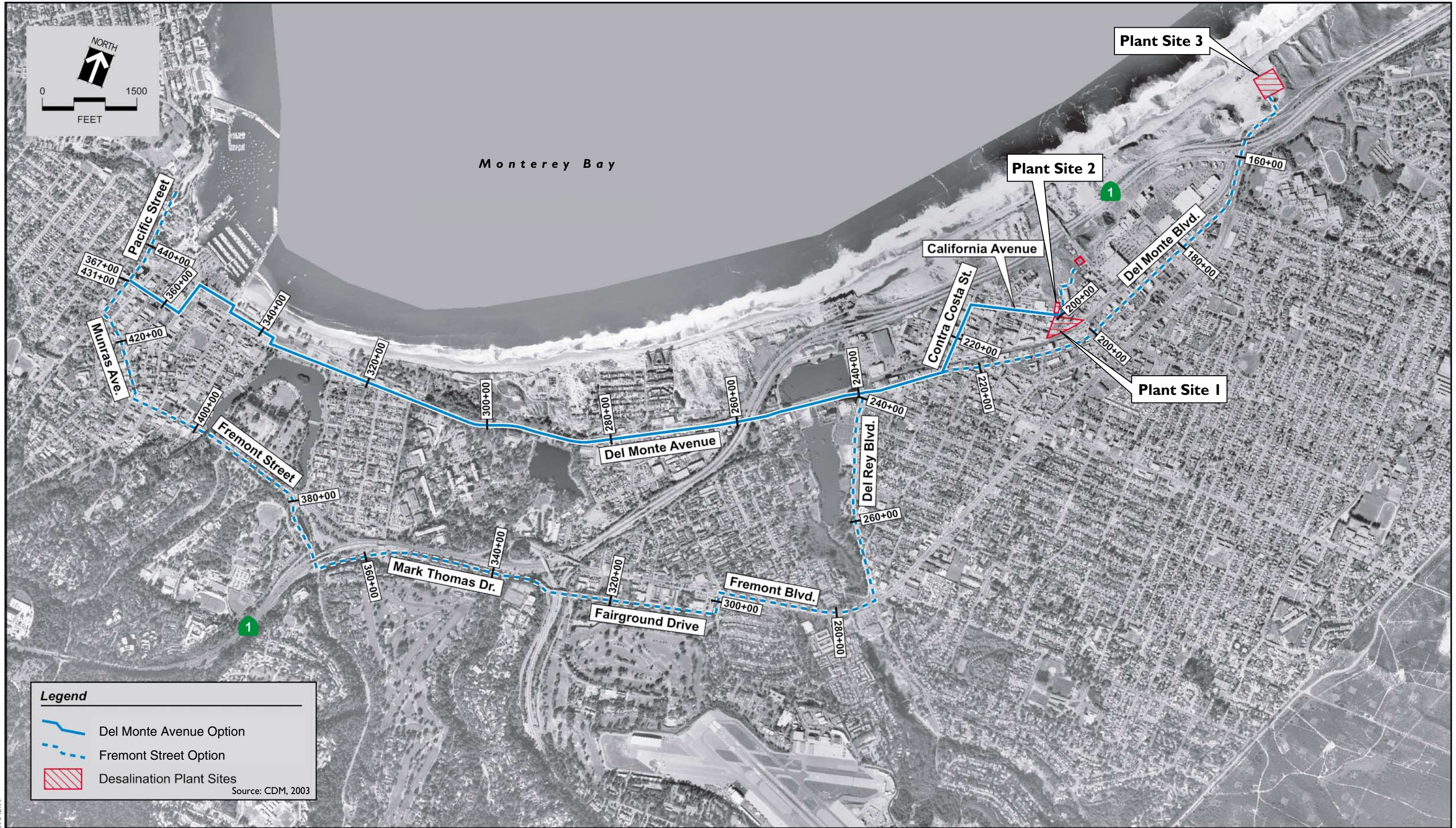
Figure ES-5 Location of Treated-Water Pipeline Options
