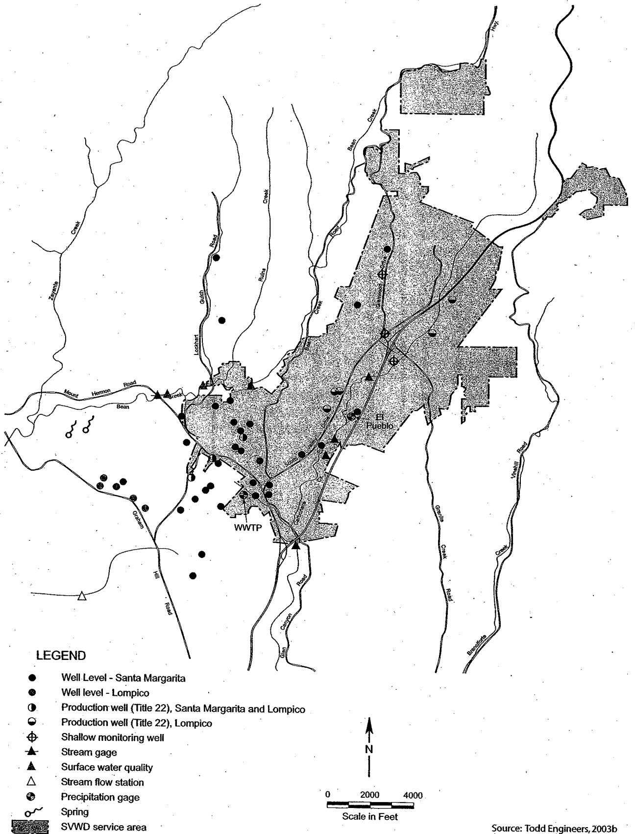
Figure 9 Scotts Valley Water District's Groundwater Management Plan monitoring locations
