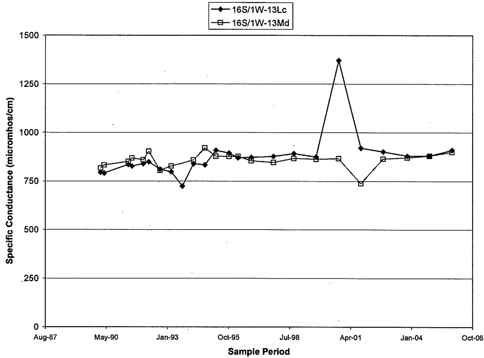
Specific Conductance in Two Wells in Carmel Valley (February 1990 through November 2005)
