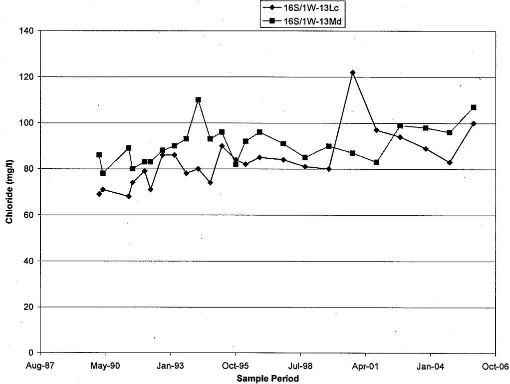
Chloride Concentration in Two Wells in Carmel Valley (February 1990 through November 2005)
