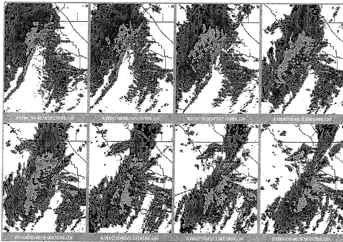
Figure 1. Convective band(s) passing over Santa Barbara County on February 2, 2004. Image times are 1436, 1459, 1528, 1609, 1632, 1701, 1730, and 1753 PST (from NAWC report on cloud seeding for SBA County).
