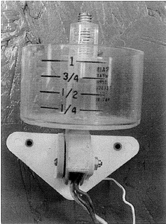
Figure 1. Weight-based rain shut-off device.
