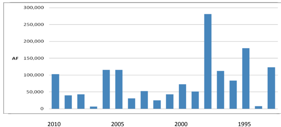
Figure 4-5. Total Annual Flows at the Carmel River/Hwy 1 Bridge (2010-1993) (AF)
