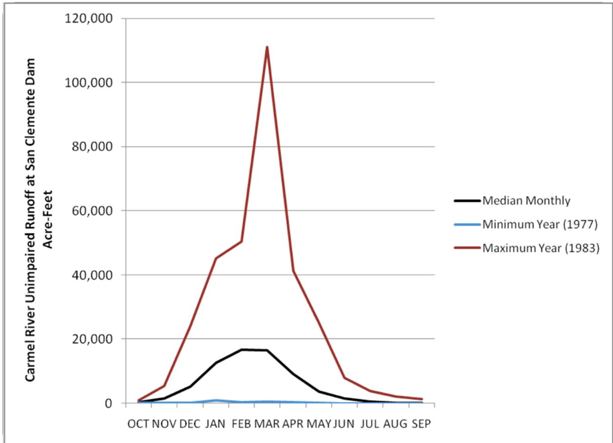
Figure 4-11. Monthly Unimpaired Carmel River Runoff at San Clemente Dam
