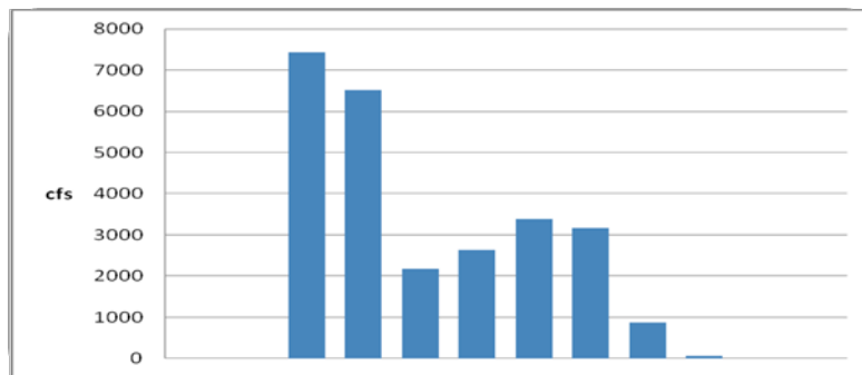
Figure 4-6. Total Monthly Flows at the Carmel River/Hwy 1 Bridge in a Normal Water Year (2003) (cfs)
