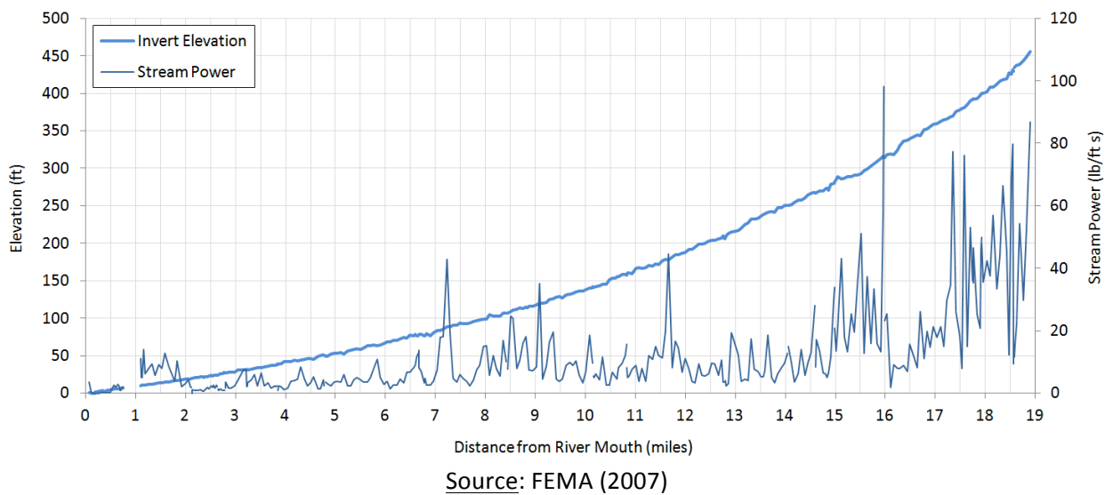
Figure 4-22 Invert profile and Total Stream Power for 100-yr flood
