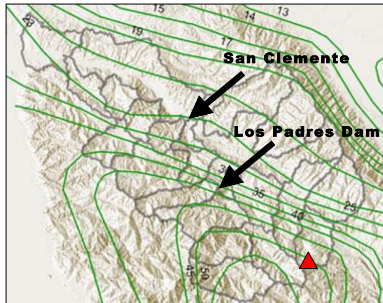
Figure 4-4. Annual Average Isohyets for the Carmel River Watershed
