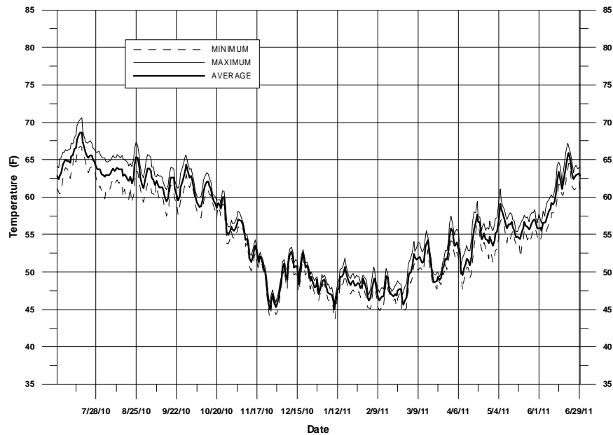
Figure III-3 Daily temperatures recorded from a continuous temperature data logger at the Sleepy Hollow Weir (SHW) station during RY 2011
