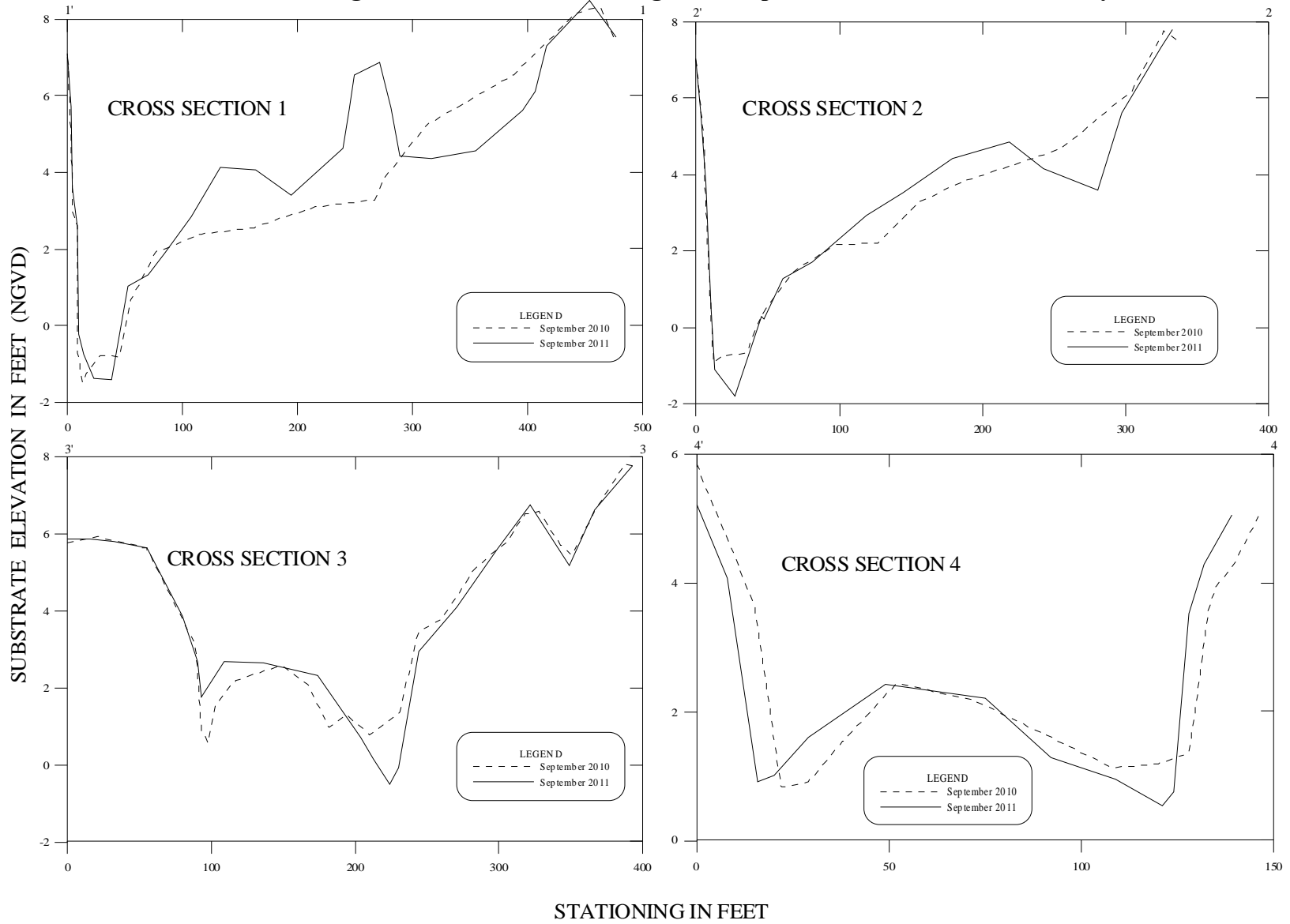
Figure XVIII-3 Carmel River Lagoon Cross Sections 1 through 4, Comparison of 2010 and 2011 Surveys
