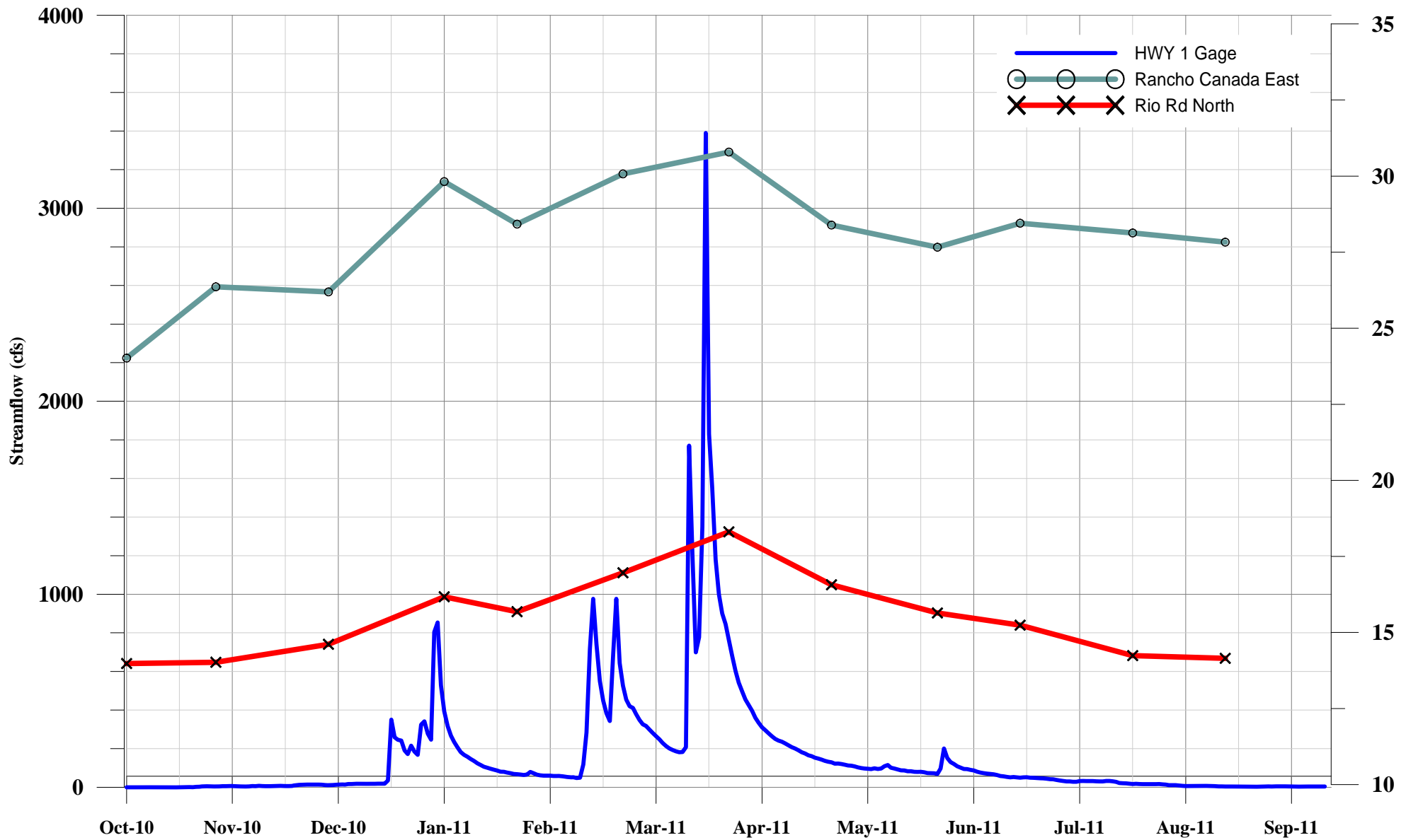
Figure IV-1 Rancho Canada East and Rio Rd North Monitor Well Water Levels and Streamflow Measured at HWY 1
