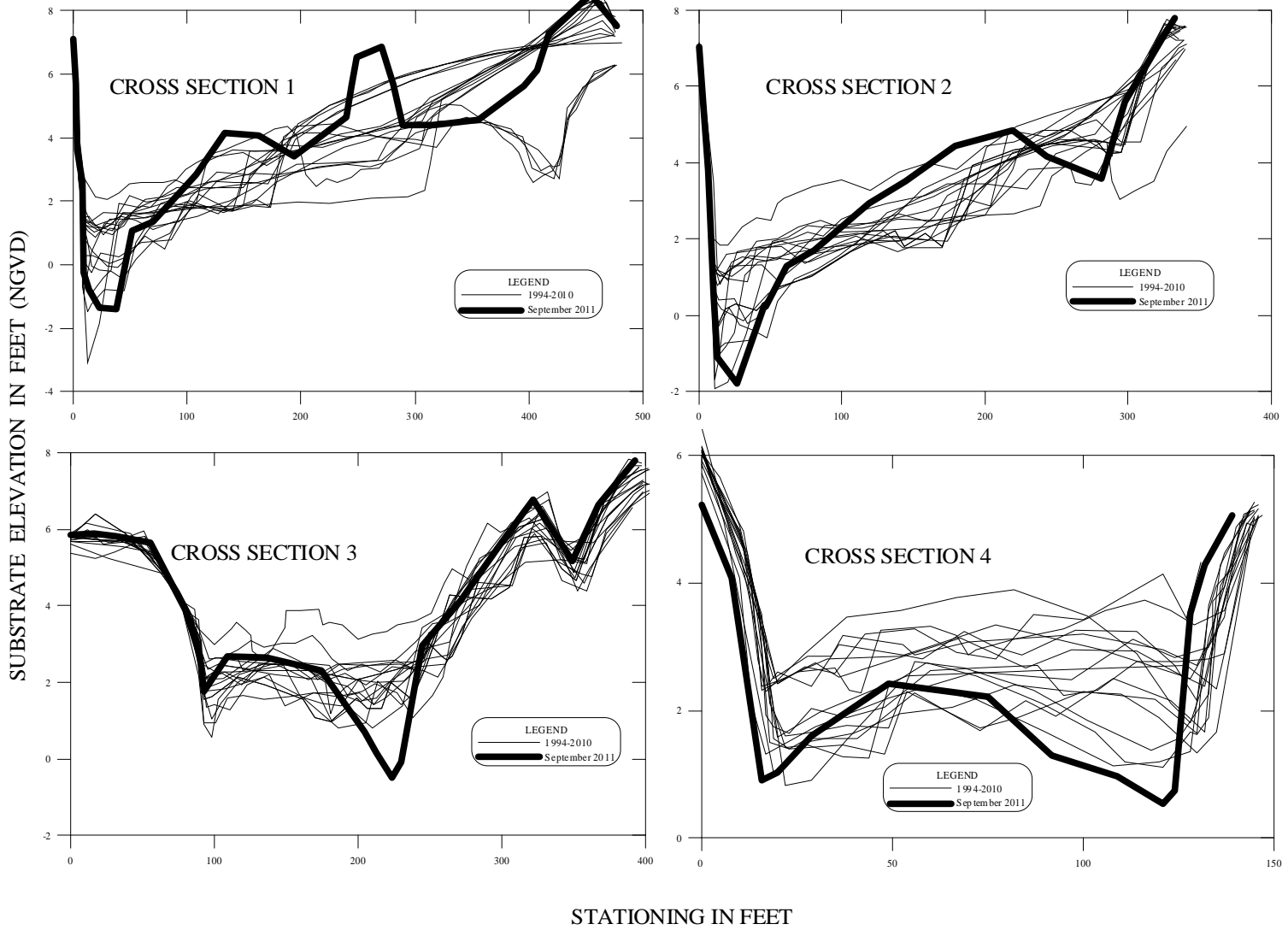
Figure XVIII-2 Carmel River Lagoon Cross Sections 1 through 4, based on Annual Surveys 1994-2011
