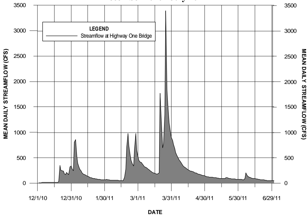
Figure XVI-2 Flow at the Highway 1 Bridge. December 2010 - July 2011
