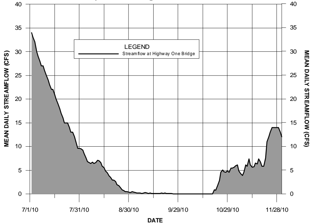
Figure XVI-1 Streamflow in the Carmel River at the MPWMD Highway 1 gaging station. July 2010 through November 2010.
