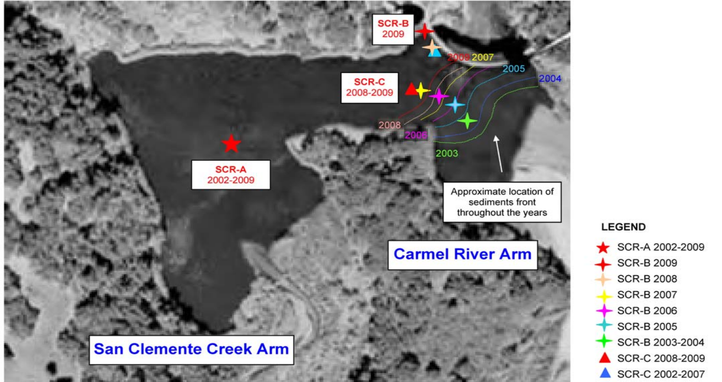
Figure 5-1 Estimated Locations of Water Quality Monitoring Stations SCR-A, SCR-B and SCR-C and Sediment Front in the San Clemente Dam Reservoir during the 2003 to 2009 Drawdown Operations
