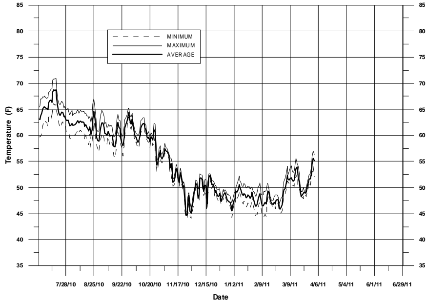
Figure III-5 Daily temperatures recorded from a continuous temperature data logger at the Below Los Padres (BLP) station during RY 2011
